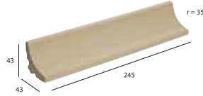
ANGULO CURVO (AC) FLOOR LEVEL UNION
