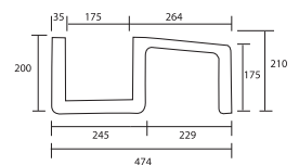
SOPORTE REJILLA (SR) GRID SUPPORTING TILE
