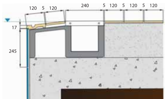
CARTABÓN EXTERIOR (CE) EXTERNAL MITERED CORNER (CE)
