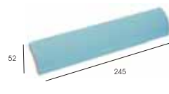
MEDIA CAÑA (MD) * RADIAL TILE
