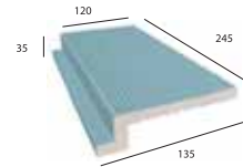
SOPORTE REJILLA (SR) GRID SUPPORTING TILE
