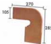
ZANQUÍN CLASSIC
